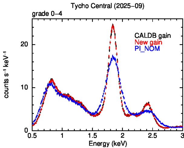
Figure C.5: Comparison of the observed and trap-corrected PC grade 0 – 4 spectra of the Tycho SNR taken in 2025-September, showing the improvements obtained when trap corrections are applied. The FWHM of the Si-K \alpha line is 258 \pm 25 eV for the uncorrected spectrum (blue) and 171 \pm 15 eV for the trap-corrected spectrum using the new gain (red), compared with 174 \pm 15 eV with the previous gain (black).
