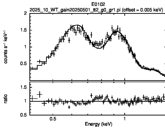
Figure C.9: WT mode spectrum of E0102 used to calibrate the low E energy scale, fitted with its IACHEC model. In previous years, N132D was also observed and analysed.
