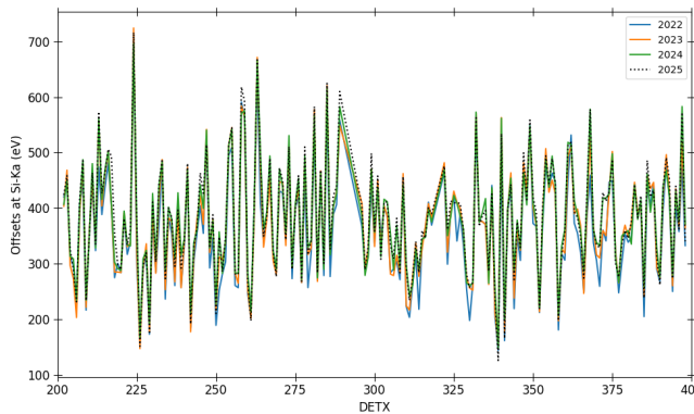
Figure C.7: Column-by-column trap depths measured from the middle Cas A pointings in 2022 (blue), 2023 (orange), 2024 (green) and 2025 (black dashed).
