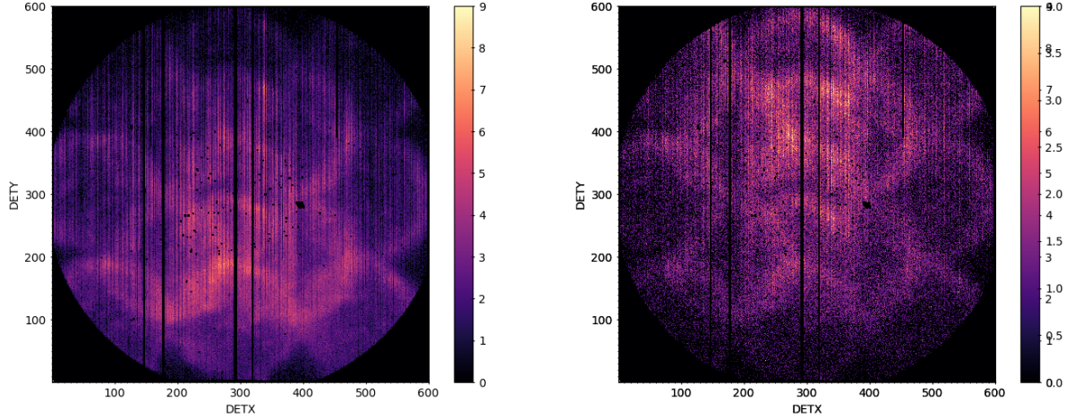
Figure C.1: Merged PC mode data of the Tycho SNR from 2023 – 2026 (exposure 1.0 Ms) showing the spatial coverage of the trap mapping observations. The left panel shows grade 0 (i.e. single pixel) events and the right panel grade 1 (i.e. vertically up-split) events. Note the reduced intensity vertical striations in some columns in grade 0, which appear as corresponding enhanced intensity striations in grade 1, are caused by grade migration as the deepest traps release charge into trailing pixels when the CCD is clocked out in the parallel direction.
